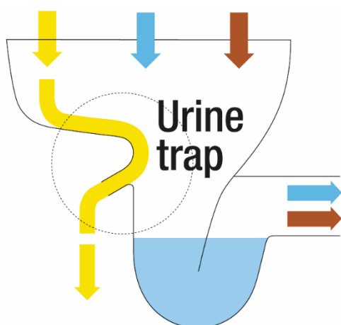
Figure 2 Basic principle of urine-separating flush toilets using the teapot effect. Copyright EOOS.
