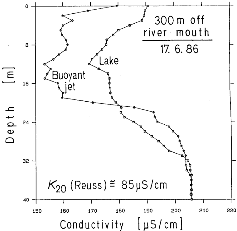
Figure 5. Electric conductivity of lake water \kappa_{20} measured at mouth of river Reuss (station U4), June 17, 1986. The spreading of the river water in the top 20 m can be traced by a drop in \kappa_{20} in the lake. Note that the river water has a significantly lower \kappa_{20} . This situation is typical for late spring and early summer.
