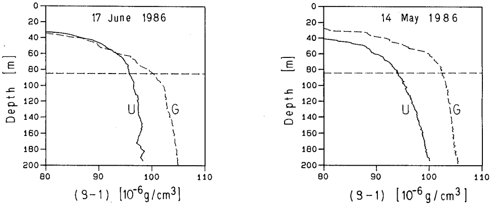
Figure 11. Density profile in Urnersee (U) and Gersauersee (G), calculated from water temperature and electric conductivity \kappa_{20} using eq. (2). On May 14, the density in G at sill depth (85 m; broken line) was larger than density at any depth in U. On June 17, the densities were equalized in most of the water column above the sill.
