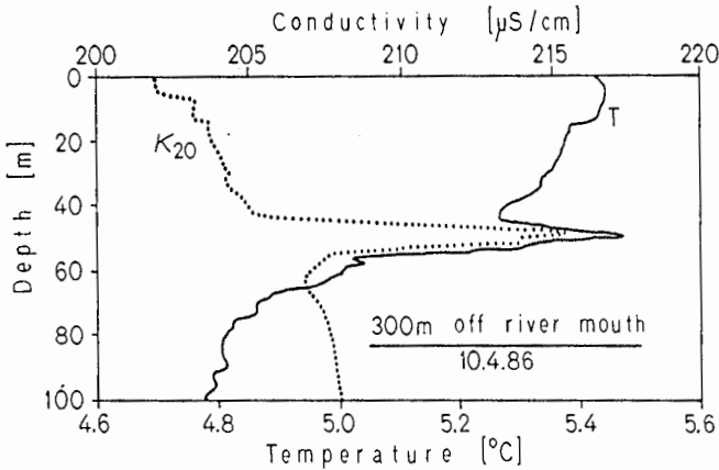
Figure 7. In April, temperature differences between river and (nearly homogeneous) lake water are still small. Therefore, small changes in the river water temperature can significantly alter the intrusion depth. On April 10, 1986, the plume from the river Muota was clearly visible at about 50 m depth. The fine structure of the temperature profile may show relicts of preceding intrusions at other depths.
