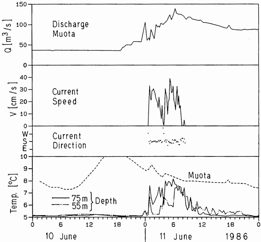
Figure 8. Density current 300 m off the mouth of river Muota on June 11, 1986, one typical example out of 9 similar events produced by heavy rainfall or thunderstorms in the drainage area (Tab. 4). Current speeds and water temperature were measured by moorings at station U1. Currents and temperature suddenly increased to maximum values of 40 cm/s and 8°C, once the river discharge exceeded about 60 m 3 s -1 . Currents point southwards into Urnersee. Fluctuation in water temperature during the event indicate changing depth of river intrusion, possibly due to changing load of suspended solids.
