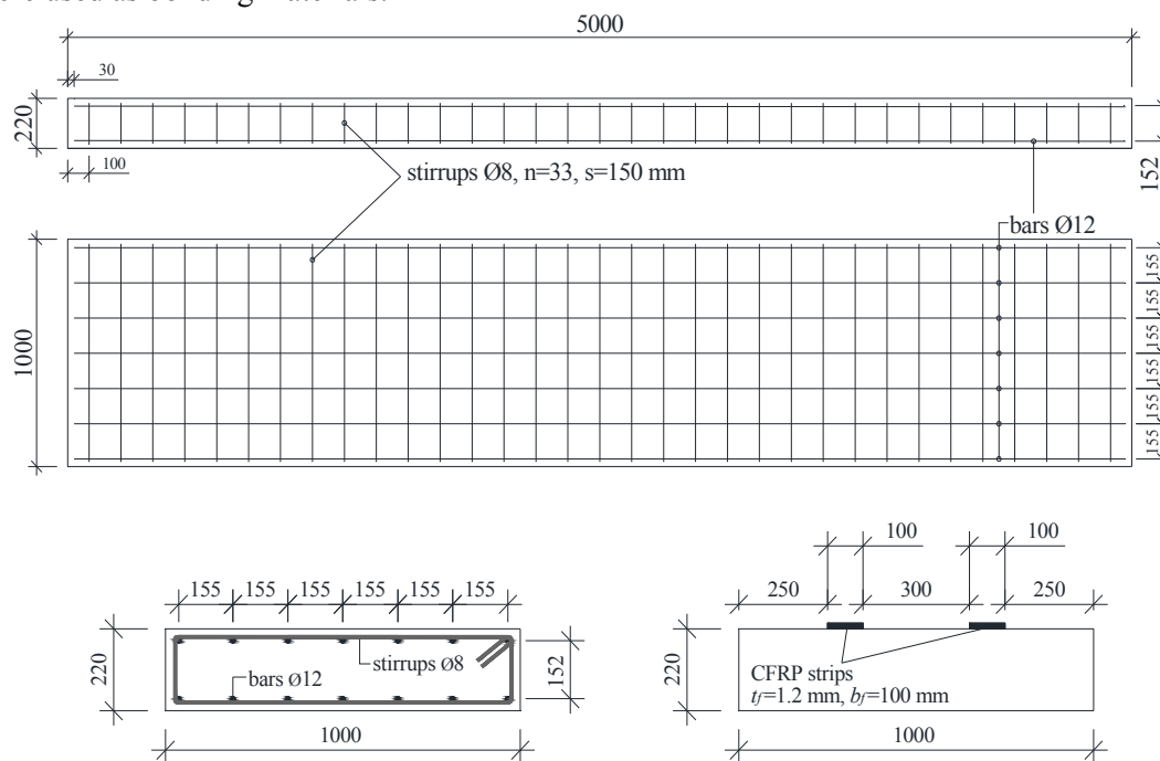
Figure 2. Geometry of the slabs and distribution of the steel reinforcement.
