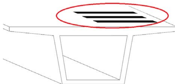
Figure 1. RC box-girder bridge strengthened in transverse direction with EB CFRP strips
