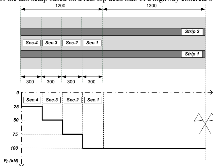
Figure 3. Sketch of the test setup based on a real top deck slab of a highway concrete box-girder bridge.
