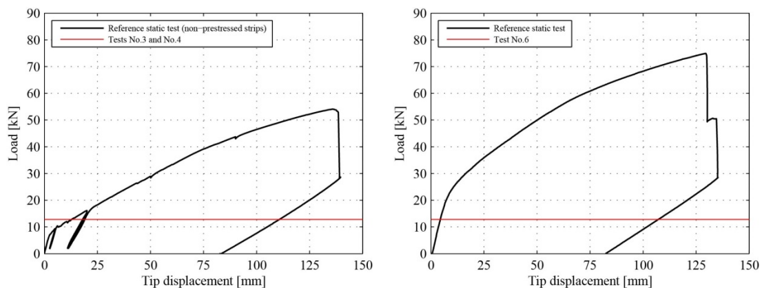
Figure 6. Load level: (Left) Strengthened slabs with non-prestressed strips and mastic asphalt (Slabs No.3 and No.4); (Right) Strengthened slab with prestressed strips and without mastic asphalt (Slab No.6).
