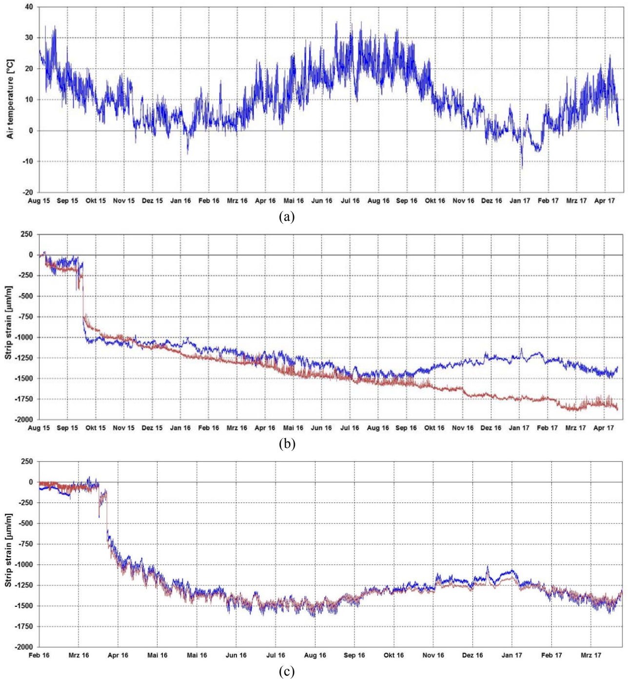
Figure 7. Experimental measurements: (a) Air temperature in shade (b) Maximum strip strains in Slab No.3; (c) Maximum strip strains in Slab No.4.
