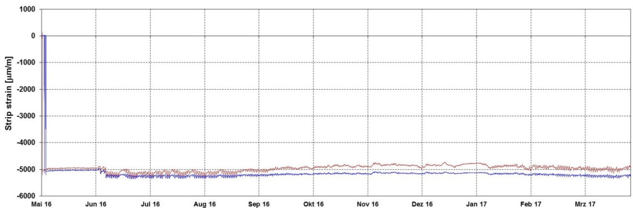
Figure 8. Experimental measurements of the strip strains in Slab No.6: Maximum strip strains.
