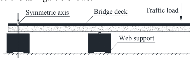
Figure 3. Sketch of the test setup based on a real top deck slab of a highway concrete box-girder bridge.
