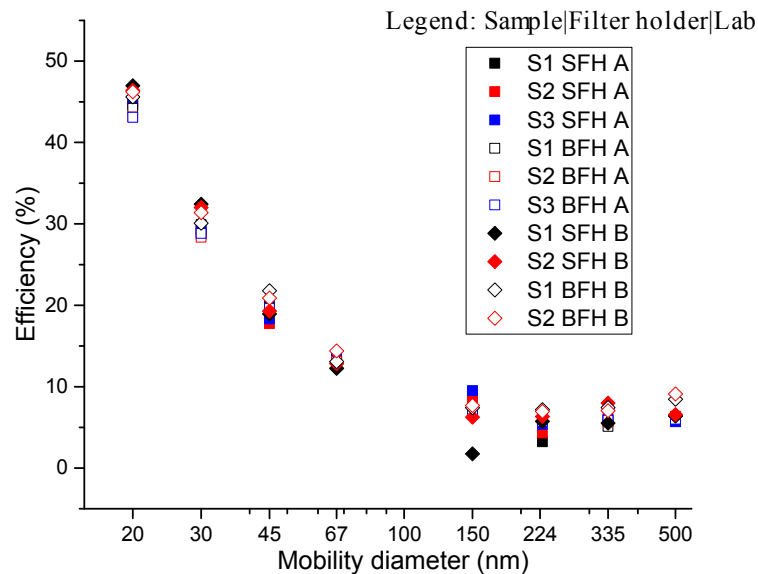
Fig. 6. Filtration efficiency of the wire mesh at 5 \text{ cm s}^{-1} measured in filter holders with different areas (SFH: Small Filter Holder, BFH: Big Filter Holder).
