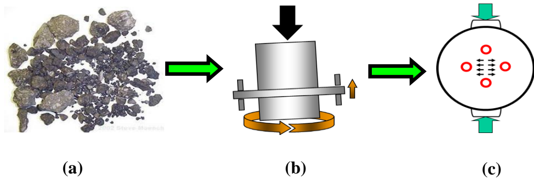
15 Fig. 1 Procedure and apparatus used in the cohesion test
