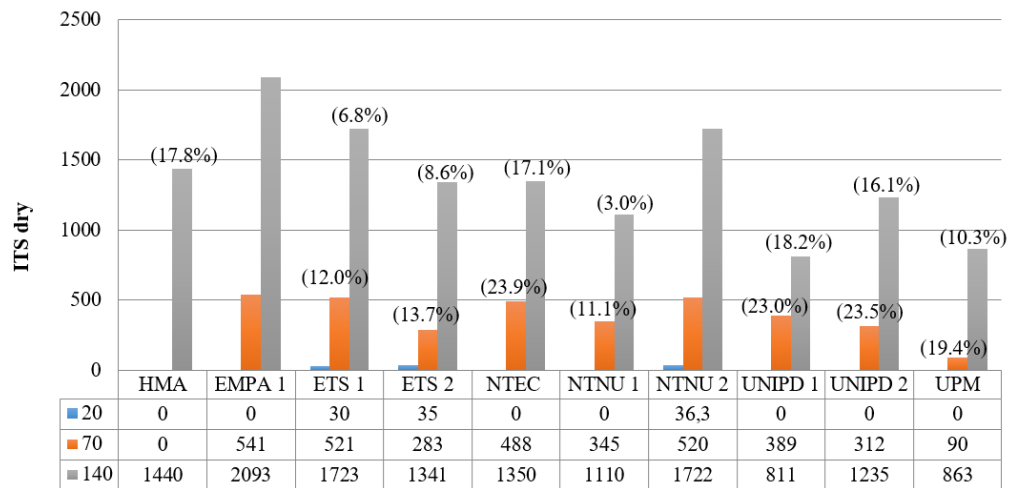
12 Fig. 3 Cohesion test results - DRY condition
