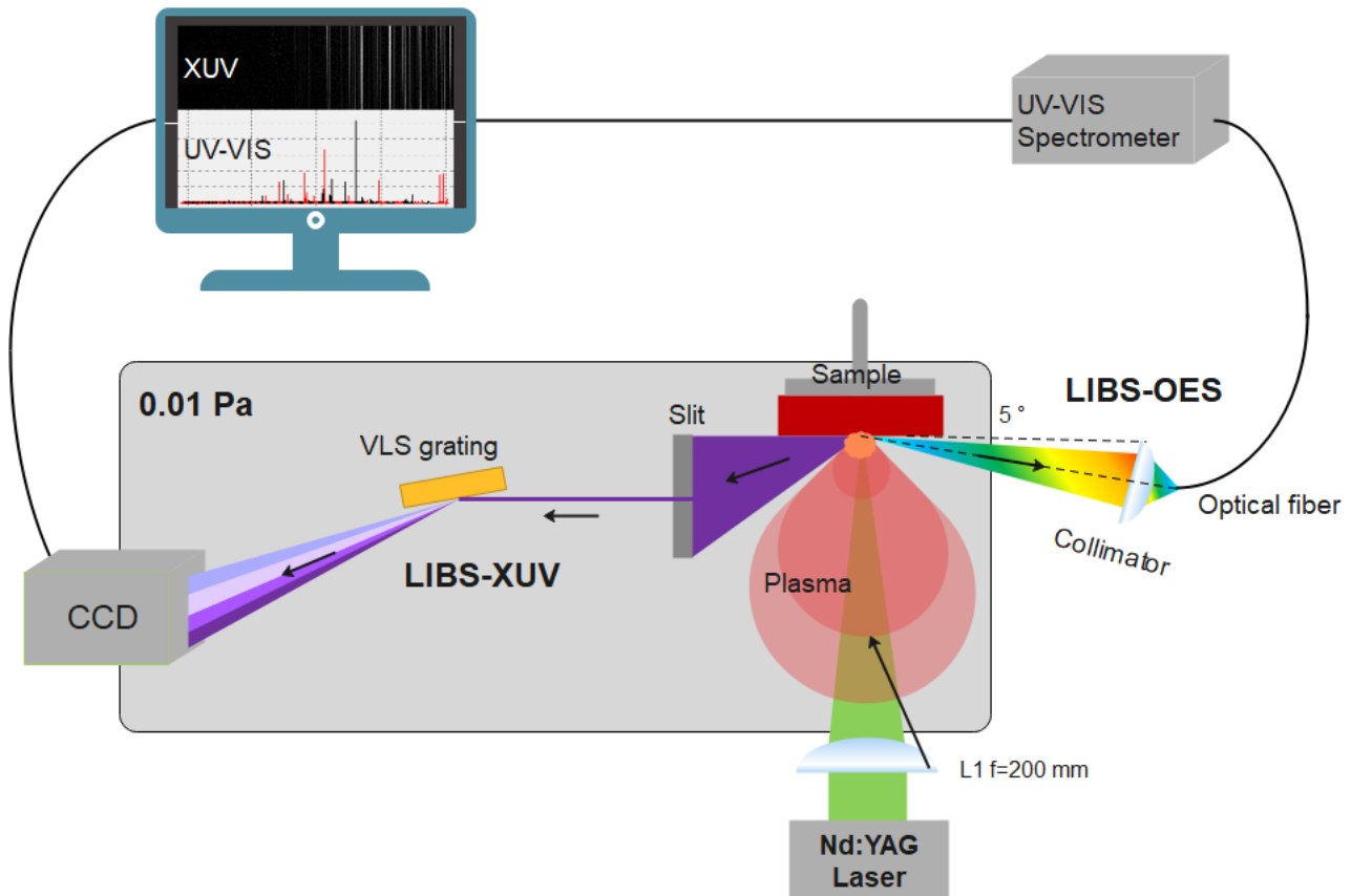
Figure 1 The LIBS-XUV and LIBS-OES setup. The laser beam ( \lambda = 532 \text{ nm} ) is focused with a lens (L1) placed in the air. The target material and XUV spectrometer are placed in the vacuum chamber. The LIBS-OES signal and LIBS-XUV signal are collected radially with a fiber optic and flat-field XUV spectrometer, respectively.
