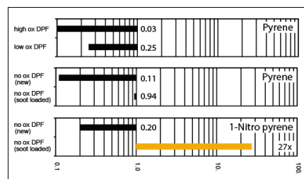
Fig. 3. Pyrene and 1-nitro pyrene penetration of filters with high, low and no oxidation potential (new and soot loaded) are compared.
