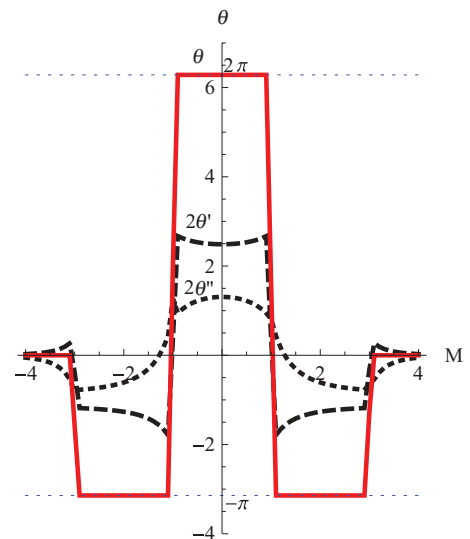
FIG. 3. (Color online) Numerical evaluation of the topological invariant \theta^{(0)} = \pi \nu(M) (solid line) for the model (III A) The parameters \theta' and \theta'' that sum up to the topological invariant \theta are defined in Eqs. (C8a) and (C8d), respectively.
