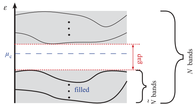
FIG. 1. (Color online) Assumed spectral gap in the single-particle energy spectrum. Here, \mu_c denotes the chemical potential and the insulating noninteracting many-body ground state |\Phi\rangle is obtained by filling all the states in the \widetilde{N} bands below the spectral gap.
