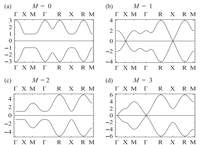
FIG. 2. Energy spectrum of the lattice model defined in Eq. (3.21) for different values of the parameter M . Panels (b) and (d) show the gap-closing topological transitions. Note the dispersionless band at zero energy in each spectrum. The spectrum is plotted along the straight path connecting the following points in the BZ: \Gamma = (0, 0, 0) , X = (0, \pi, 0) , M = (\pi, \pi, 0) , and R = (\pi, \pi, \pi) .
