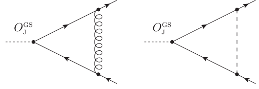
FIG. 4. One-loop diagrams contributing to the form factor \bar{F}_{q,J}^{\text{GS}} including a gluon (left) and an associated \epsilon -scalar (right). The right diagram is proportional to the evanescent coupling \alpha_e and only contributes in the FDH scheme.
