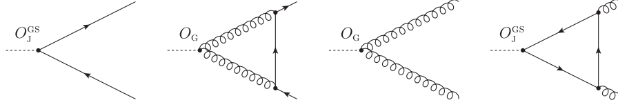
FIG. 3. Lowest-order contributions to the pseudoscalar form factors \bar{F}_{q,J}^{\text{GS}} , \bar{F}_{q,G} , \bar{F}_{g,G} , and \bar{F}_{g,J}^{\text{GS}} (from left to right). Note, that the “mixed” amplitudes \bar{M}_{q,G} and \bar{M}_{g,J} are loop induced and are therefore at least of \mathcal{O}(\alpha_s) .
