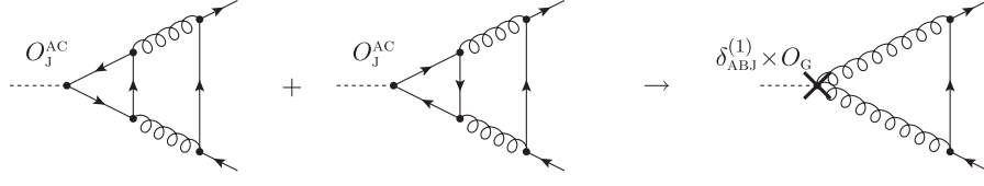
FIG. 7. Equivalence between anomalous two-loop contributions to \bar{M}_{q,J}^{AC} and \delta_{ABJ}^{(1)} \bar{M}_{q,G}^{(1)} .
