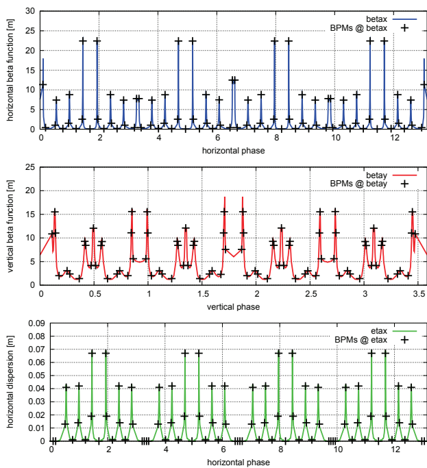
Figure 2: Photon and RF BPM layout with 20 photon and 64 RF BPMs for one 3rd of SLS-2. BPMs are visualized as “+” with the values of the corresponding beta functions and horizontal dispersion, where the total phase advance of SLS-2 (Version AD05F) is 39.417 and 10.755.
