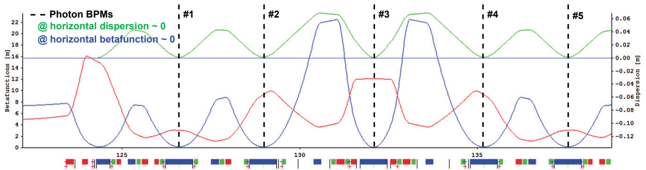
Figure 1: One arc section of the SLS-2 lattice (Version AD05F) with a schematic view of the magnets at the bottom (dipole magnets in blue) and the optical functions. The horizontal beta function (blue) and the horizontal dispersion (green) vanishes in the center of the bending magnets in order to provide small horizontal emittance. Five additional photon BPMs (#1-#5) have been added in the center of the main bends for improved orbit sampling.
