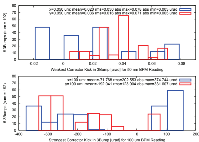
Figure 4: Graph 1: Histograms of the weakest horizontal (min \approx 3 nrad) and vertical correctors (min \approx 5 nrad) in 192 interleaved 3-bumps for a 50 nm BPM reading (BPM resolution) in the 3-bump center, Graph 2: Histograms of the strongest horizontal (max \approx 375 \mu\text{rad} ) and vertical correctors (max \approx 330 \mu\text{rad} ) for a 100 \mu\text{m} BPM reading (BPM resolution) in the 3-bump center.
