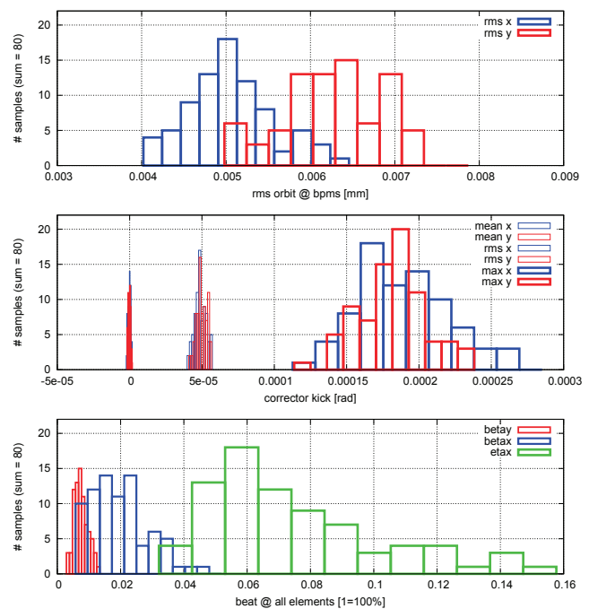
Figure 3: Graph 1: Residual horizontal (mean rms 5 \mu\text{m} ) and vertical (mean rms \approx 6 \mu\text{m} ) rms orbit taken at the locations of the BPMs for 80 error distributions (Note that the rms is non-zero since the number of BPMs exceeds the number of correctors), Graph 2: Necessary rms corrector strength (mean rms \approx 50 \mu\text{rad} in both planes, mean maximum \approx 175 \mu\text{rad} ), Graph 3: Resulting beta (mean \approx 1\text{-}2 \% in both planes) and dispersion beat (mean \approx 7 \% ).
