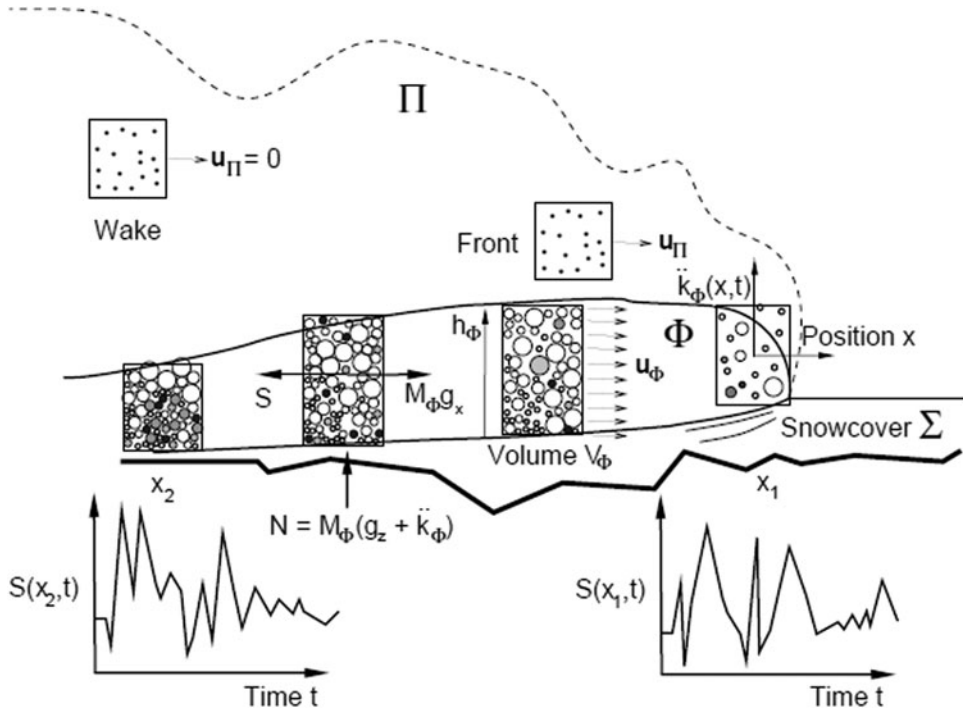
Figure 3. The avalanche core \Phi experiences a continuous series of jolts from the boundary. Shearing S(x, t) induces changes in slope-perpendicular accelerations \ddot{k}_\Phi(x, t) which are an unknown function of position x and time t . The accelerations depend on the speed of the avalanche, as well as external factors such as terrain. The configurational energy of the core R_V , and therefore flow friction, depends on the external forcing, which is a function of x and t . The component of gravity in the x -direction is denoted g_x . It acts on the core mass, not the cloud mass. Large velocity gradients exist between the leading edge and tail (wake) of the powder cloud \Pi .
