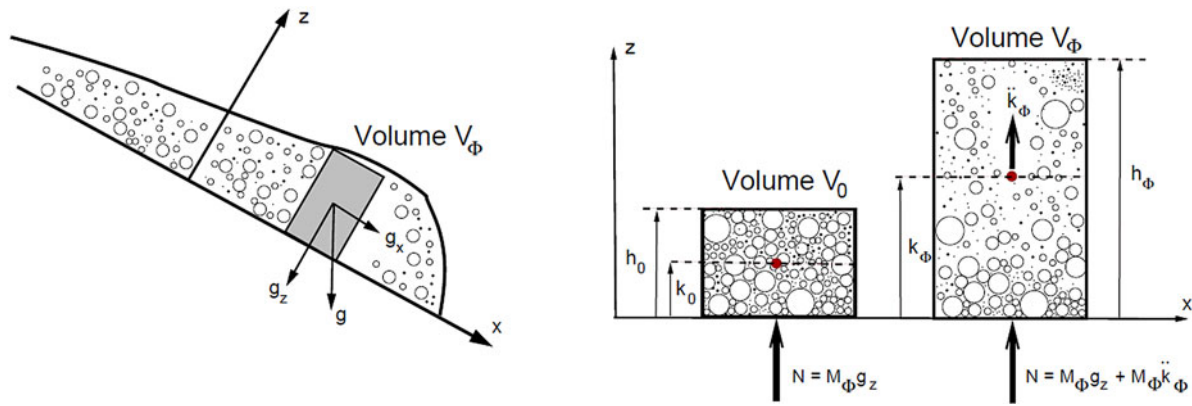
Figure 1. Newton's law of action and reaction applied to a flow column in the avalanche body. Avalanche mass flows in the slope parallel x -direction. The column can expand in the slope perpendicular z -direction. Particulate avalanche mass M_\phi flows through the column; the column sides are fixed and therefore the volume V_\phi can only vary with height. We consider two states: (a) the co-volume, or dense packing of snow granules. The norm of the force on the ground is N = M_\phi g_z . The center-of-mass of the co-volume is located at k_0 . (b) During flow the particulate mass M_\phi is sheared and expands due to the acceleration \ddot{k}_\phi . The height of the flow column, defined by the location of the highest particle, is now h_\phi . The center-of-mass moves from k_0 to k_\phi . The reaction to the acceleration of the center-of-mass is termed the dispersive pressure N_k = M_\phi \ddot{k}_\phi . No restrictions are made on the timescale of the expansion.
