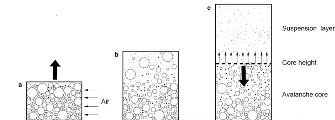
Figure 6. Our model decouples the suspended and heavy mass, allowing the modeling of both the avalanche front and avalanche wake without imposing artificial interfaces. The avalanche core is defined by the location of the highest heavy particle. This mass never leaves the core, but expands upwards into the suspension layer, often to great heights. Momentum is transferred from the heavy particles to the air giving the suspension layer an initial velocity (initial condition).
