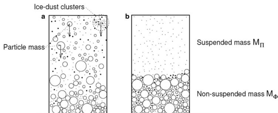
Figure 4. A representative column in the avalanche. Avalanche mass is divided into suspended mass M_{II} and heavy mass that falls to the ground under gravity M_{\Phi} . The two masses (a) overlap. The suspension layer consists of suspended mass M_{II} (by definition); the avalanche core consists of the gravity driven mass M_{\Phi} . Both layers have the same height measured from the ground. (b) The heavy mass segregates out of the suspension layer. Packets of ice-dust (clusters) may fall under gravity, acting as a coordinated whole and thus belong to the core mass M_{\Phi} .
