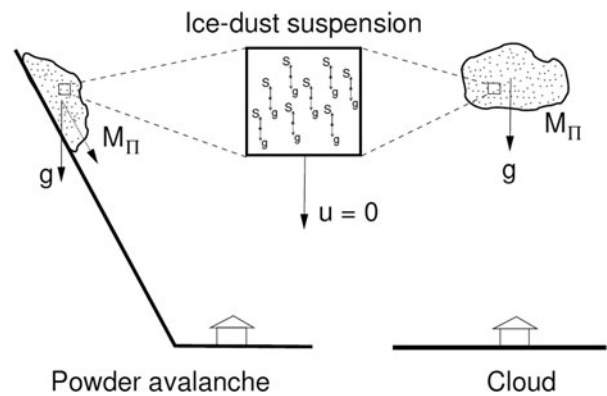
Figure 5. The model of Issler and others (2017) treats suspension clouds as gravity currents. They argue that gravity accelerates a suspension cloud because the density difference between the ice and air is large. Their model predicts, clouds should fall from the sky and reach large velocities. The inclusion of gravity in our model of the suspension cloud is in error because M_{II} contains only mass that can be suspended. That is, we assume no relative movement of the particles with the air g = S . The cloud can only move by accelerating the air containing the ice particles.
