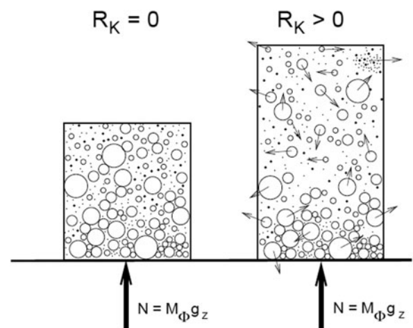
Figure 2. Two columns in the avalanche, both contain the same mass M_\phi . The avalanche column on the left contains no random energy R_K = 0 ; the column on the right contains random energy R_K > 0 . Only when the center-of-mass of the column changes, there will be a change in the normal pressure N . The weight of both masses remains the same N = M_\phi g_z . This is Newton's law of action and reaction. According to Issler and others (2017) the normal force N is proportional to R_K .
