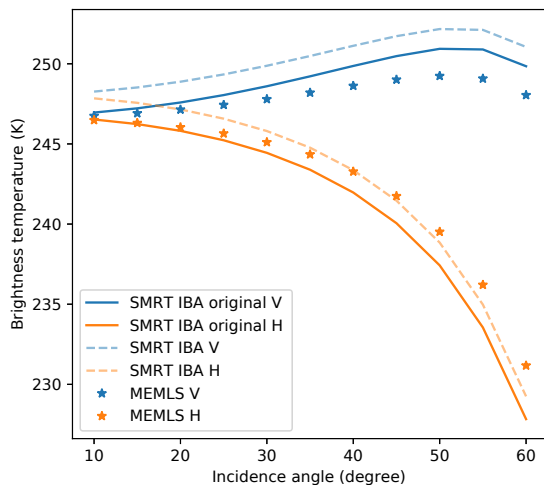
Figure 6. Comparison of brightness temperatures simulated by SMRT IBA with an exponential autocorrelation function and MEMLS. The correlation length is 100\ \mu\text{m} ; other parameters are similar to those of Fig. 4.
