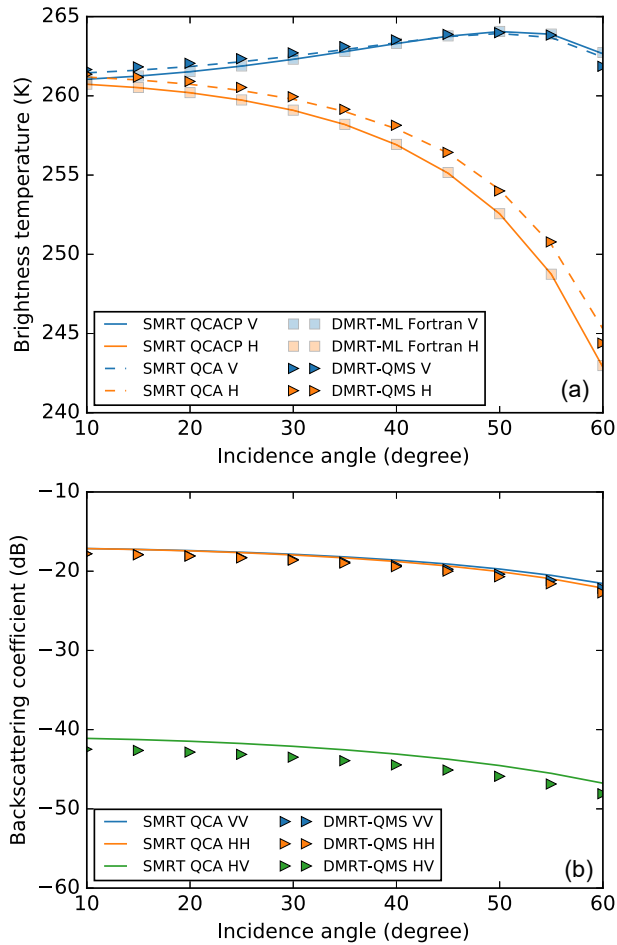
Figure 4. Comparison of brightness temperatures (a) and backscattering coefficients (b) simulated by SMRT QCA, SMRT QCA-CP, DMRT-ML, and DMRT-QMS (when relevant for the active mode). The snowpack is semi-infinite with a density of 300 \text{ kg m}^{-3} , sphere radius of 100 \mu\text{m} , temperature of 265 \text{ K} , and stickiness of 0.5 . The frequency is 37 \text{ GHz} .
