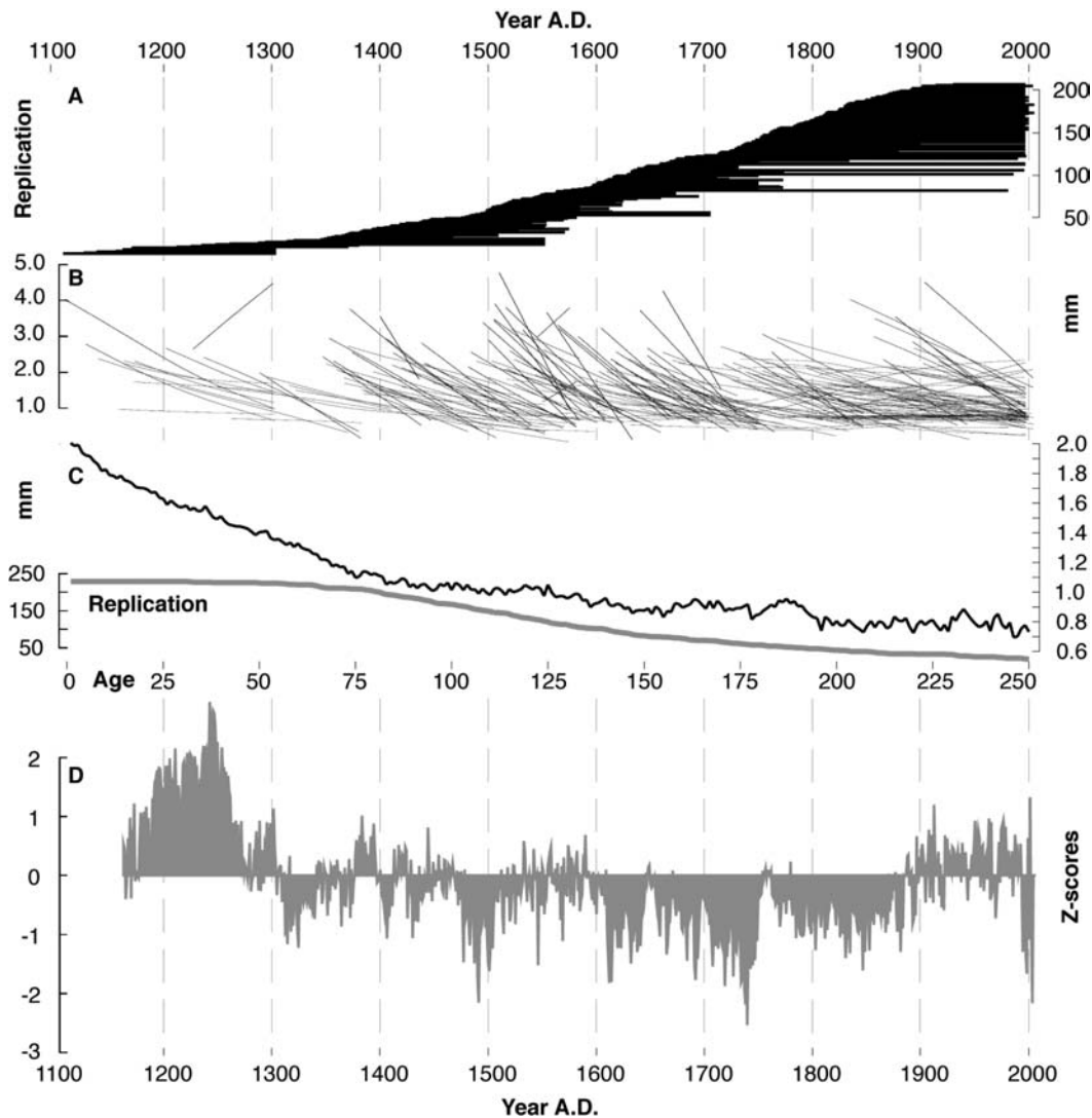
Fig. 2 A Temporal distribution of the 208 recent and historic samples. B Individual 300 year splines fit to each series. C Age-aligned mean curve ( RC , calculated after power-transformation), and their replication. D Residuals between the 300 year spline and RCS chronology
