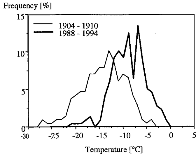
Figure 4. Frequency distribution of daily minimum temperatures ( ^{\circ}\text{C} ) for two distinct periods at Davos, Switzerland ( 46^{\circ}50'\text{N} , 09^{\circ}51'\text{E} , altitude 1590 m).
